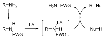
Scheme 1. Double activation of amino groups with EWG and LA.
