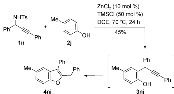
Scheme 3. One-step synthesis of benzofuran 4nj .
