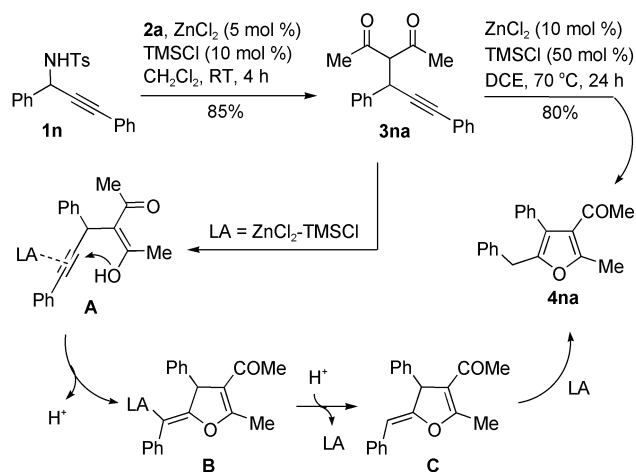
Scheme 2. Cycloisomerization of \beta -alkynyl diketone 3na to generate furan 4na .
